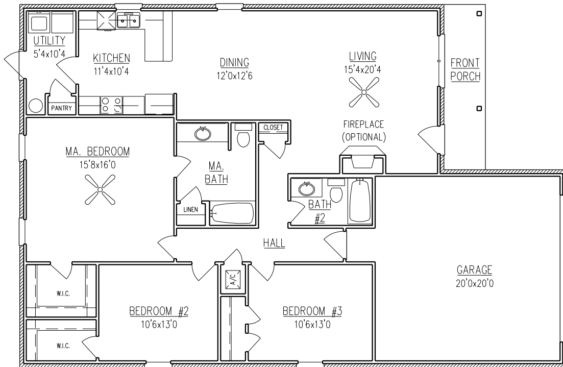
FLOOR PLAN
